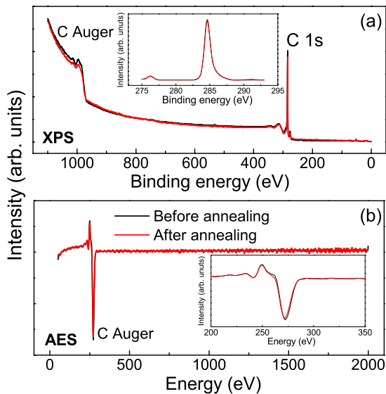
FIG. 2. (Color online). (a) XPS spectra before and after annealing. (b) AES spectra before and after annealing. Insets: magnified carbon peaks.
