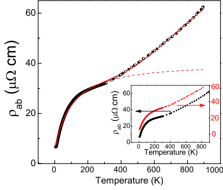
FIG. 1. (Color online). Measured temperature dependence of the in-plane resistivity of HOPG for warming (filled squares) and cooling (blank squares) temperature sweeps. Dashed: theoretical prediction for \rho_{ab}(T) in the model containing scattering at impurities and soft phonons. Solid: fit using the model containing scattering at impurities, soft phonons, and intervalley scattering at hard in-plane optical phonons [Eq. (17)]. Inset: overlap of the data for two different samples. The vertical scales were shifted for clarity.
